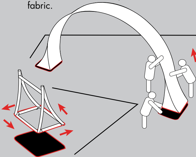
Detail shown without main Rib Arch fabric.
